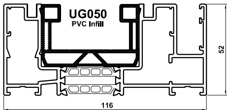
VG511 Two Track Outer Frame with Internal Upstand
