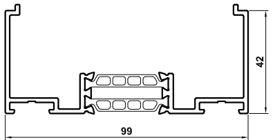
VG558 VG510 Head Extension
