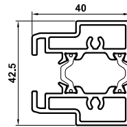
VG540 Meeting Stile Adaptor
