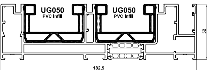
VG513 Three Track Outer Frame with Internal Upstand
