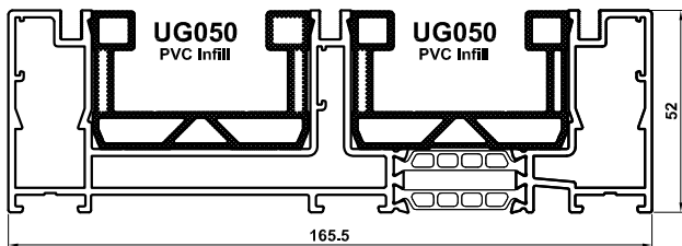
VG512 Three Track Outer Frame
