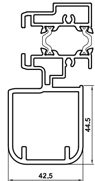
VG541 Meeting Stile Adaptor
