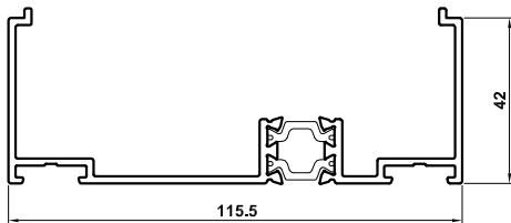
VG570 VG511 Head Extension
