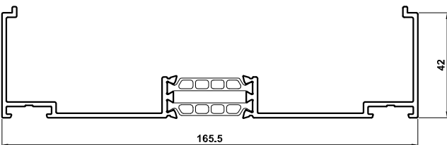
VG559 VG512 Head Extension
