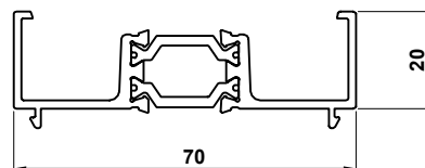
DV559 Outer Frame Extension
