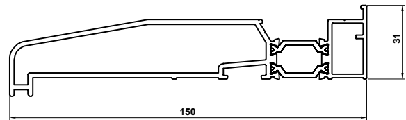
ETC457 150mm Cill
