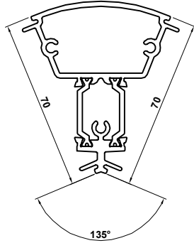
ETC385 135° Corner Post
