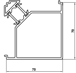
ETC048 Corner Post
