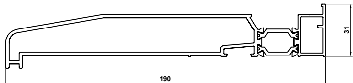
ETC458 190mm Cill
