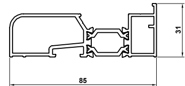
ETC451 85mm Stub Cill
