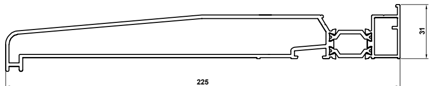
ETC479 225mm Cill
